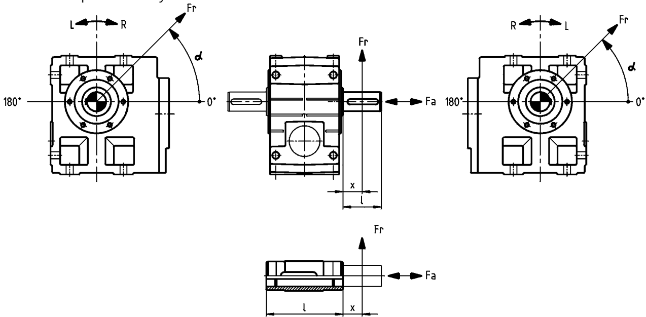
Effective direction factor f_{\alpha} at output shaft
