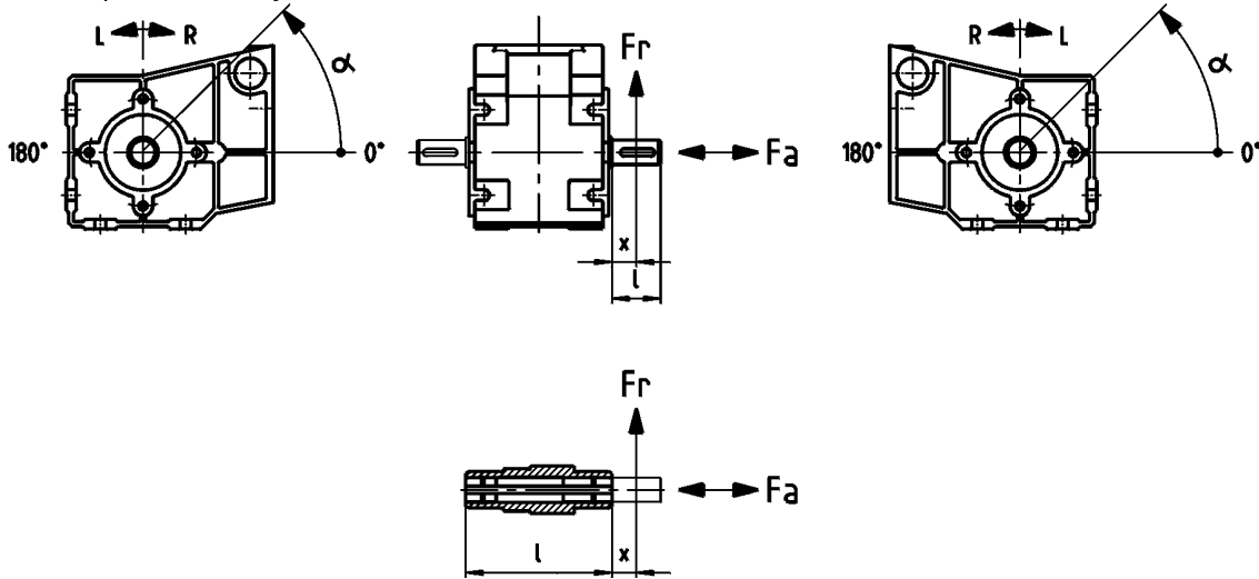
Effective direction factor f_{\alpha} at output shaft
