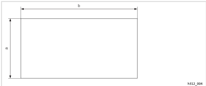
Fig. 2-3 Mounting cutout
